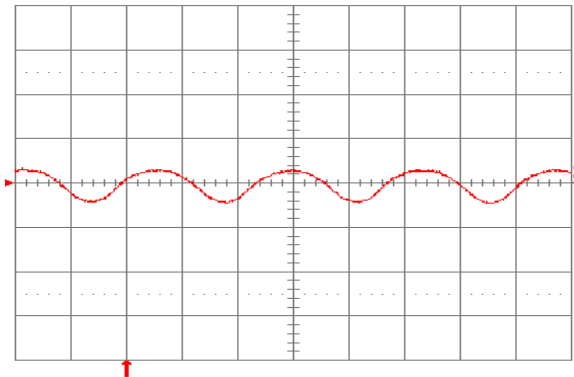
Fig. 1.5V.9: Input reflected ripple current, i_c (100 mA/div.), measured at input terminals at full rated load current and V_{in} = 48\ \text{V} . Refer to Fig. 1.5V.8 for test setup. Time scale: 1\ \mu\text{s}/\text{div} .
