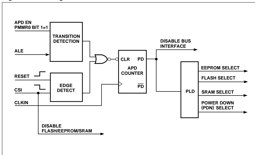
Figure 30. APD Logic Block
