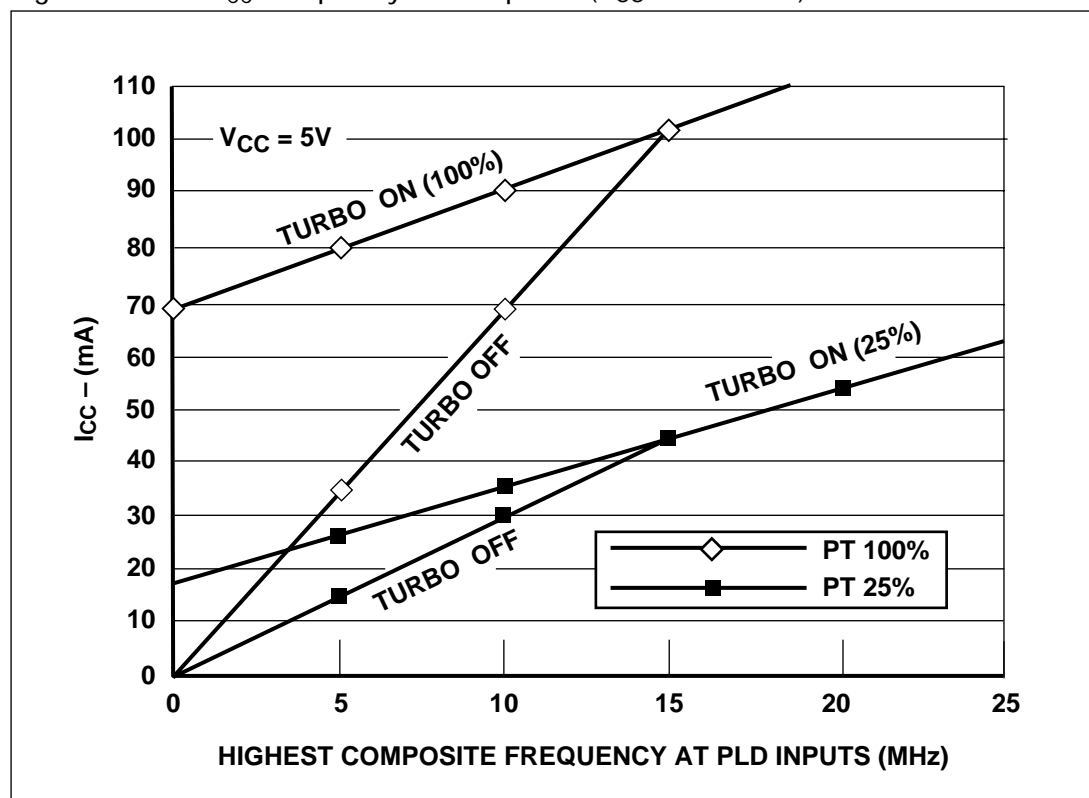
Figure 33. PLD I_{CC} /FrequencyConsumption ( V_{CC} = 5\text{ V} \pm 10\% )
