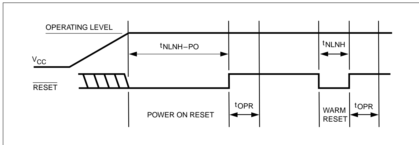
Figure 45. Reset Timing
