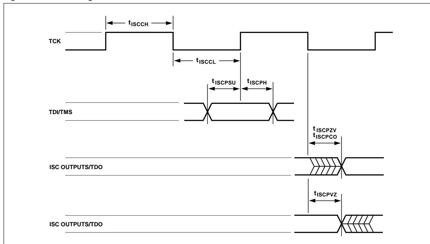
Figure 44. ISC Timing
