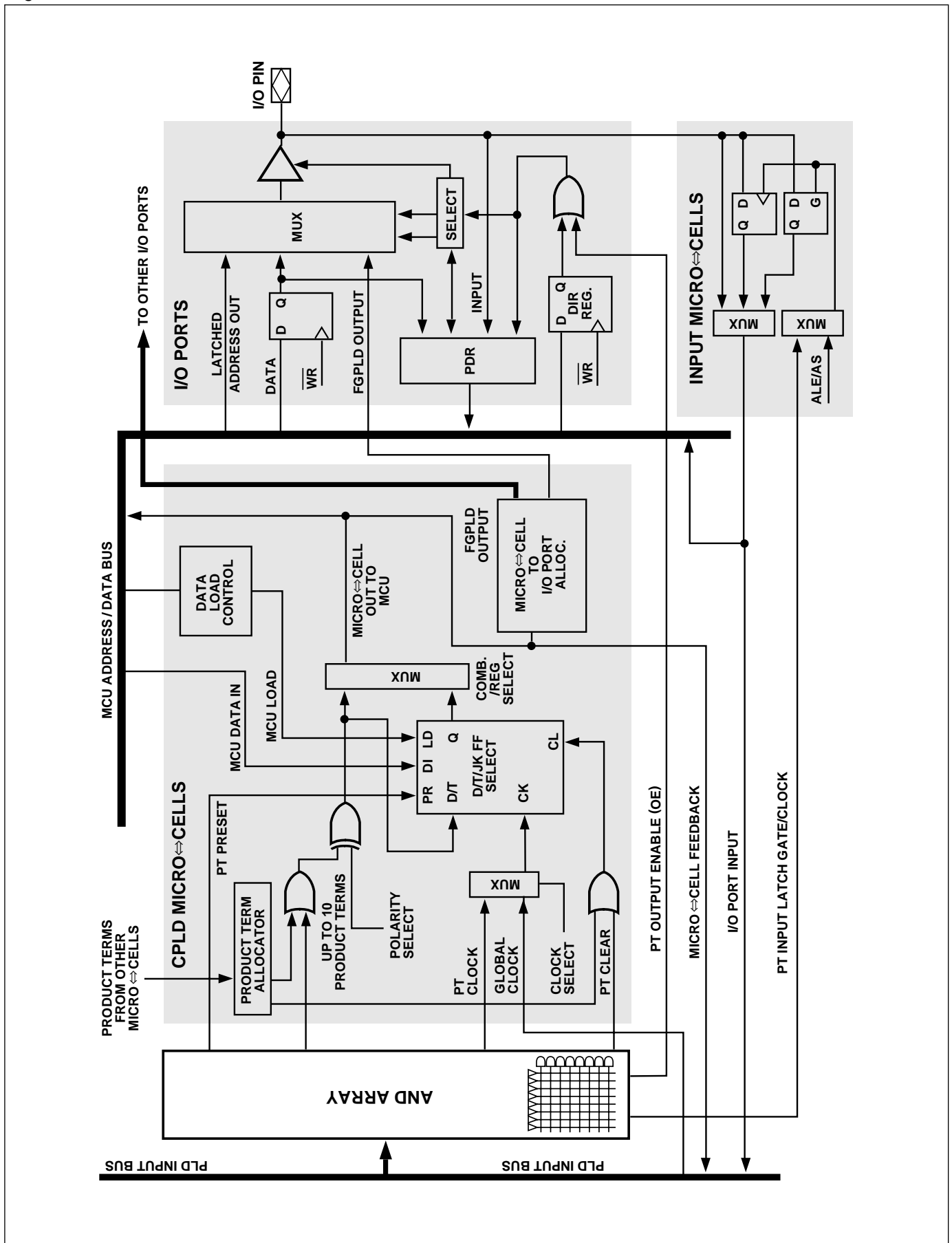
Figure 13. The Micro \leftrightarrow Cell and I/O Port
