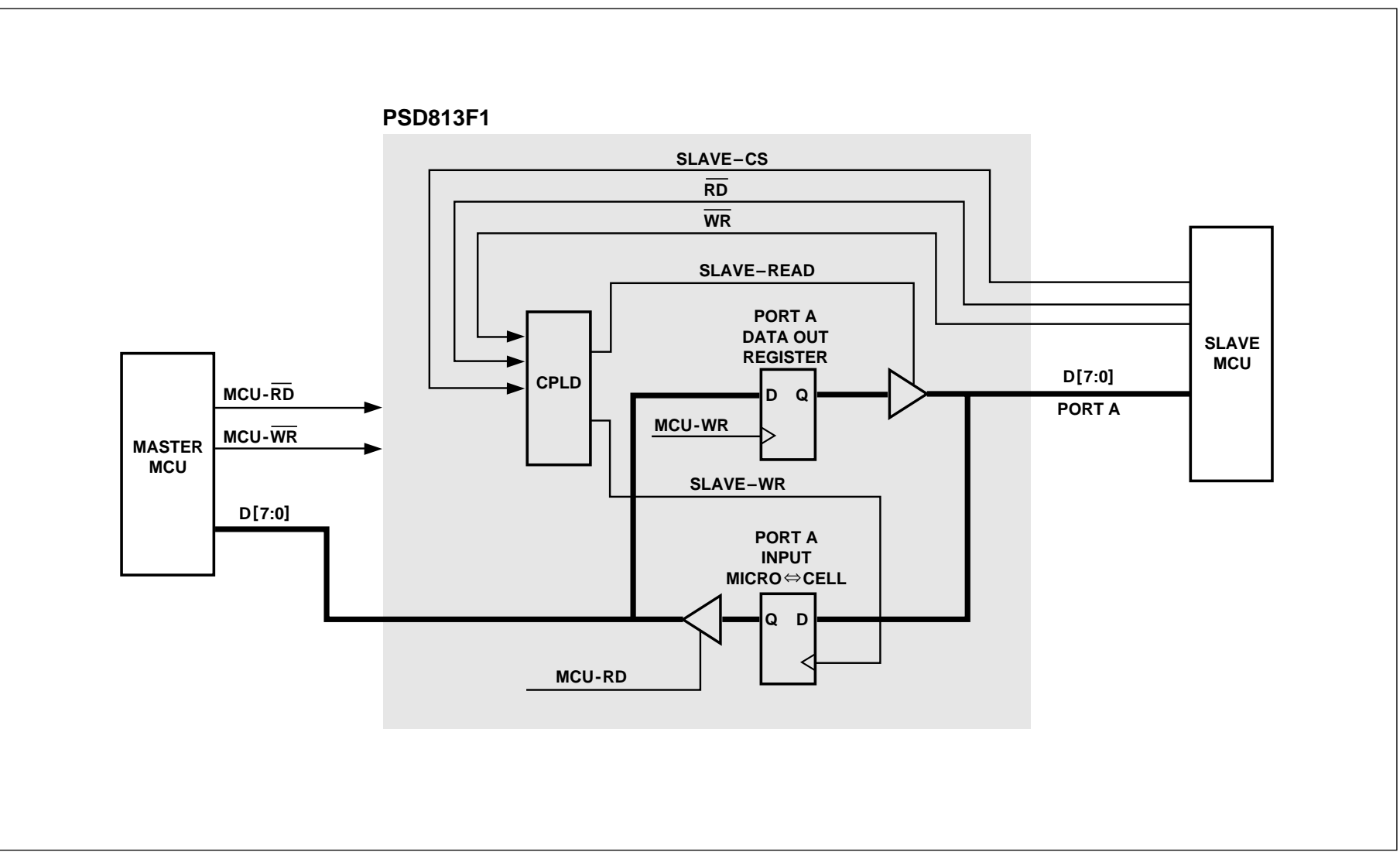
Figure 16. Handshaking Communication Using Input Micro \Rightarrow Cells
