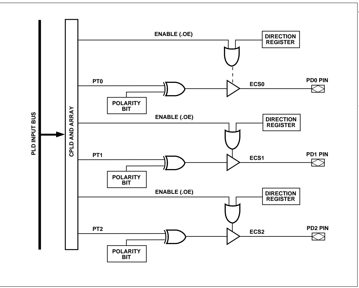
Figure 29. Port D External Chip Selects
