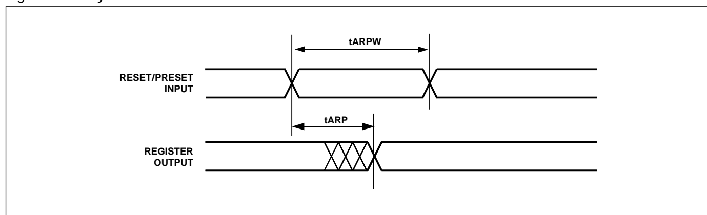
Figure 43. Asynchronous Reset/Preset
