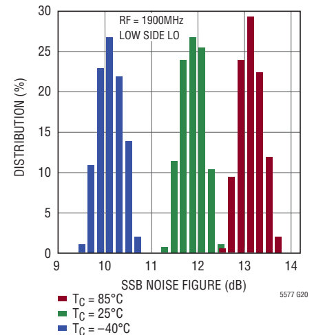
1900MHz SSB NF Distribution
