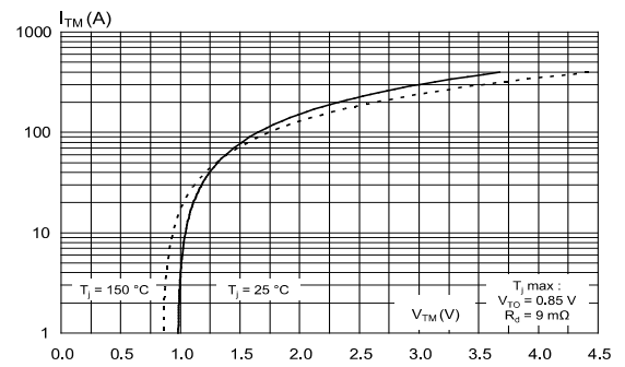
Figure 10: On-state characteristics (maximum values)
