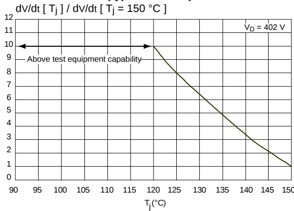
Figure 7: Relative variation of static dV/dt immunity versus junction temperature (typical values)
