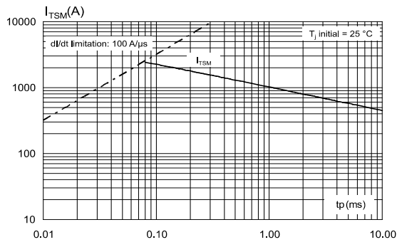
Figure 9: Non repetitive surge peak on-state current for a sinusoidal pulse with width t_p < 10\text{ ms}
