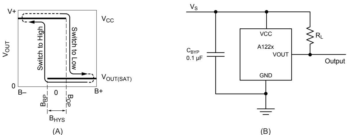
Figure 1. Switching behavior of latches. In panel A, on the horizontal axis, the B^+ direction indicates increasing south polarity magnetic field strength, and the B^- direction indicates decreasing south polarity field strength (including the case of increasing north polarity). This behavior can be exhibited when using a circuit such as that shown in panel B.
