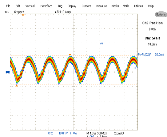
Fig. 20: Output Voltage Ripple, 12A load Ch_2: V_{out}
