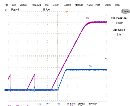
Fig. 22: Short (Hiccup) Recovery Ch_1: V_{out} , Ch_3: V_{ss}
