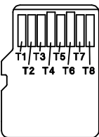
microSD CARD
