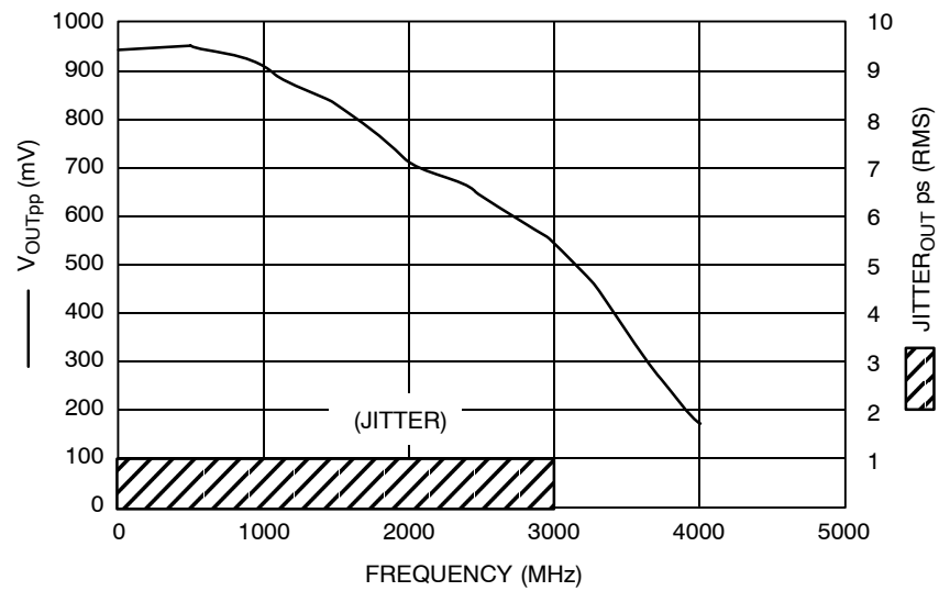
Figure 4. F_{max}/Jitter
