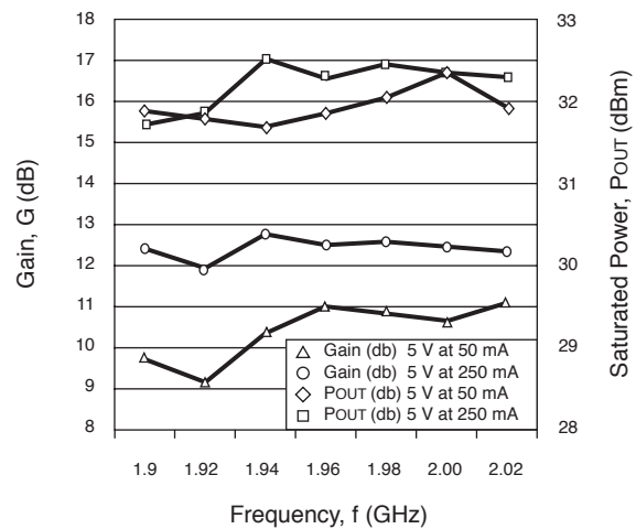
GAIN AND SATURATED POWER vs. FREQUENCY
