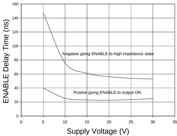
ENABLE Propagation Time vs. Supply Voltage
