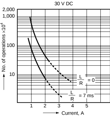
1. Life curve
