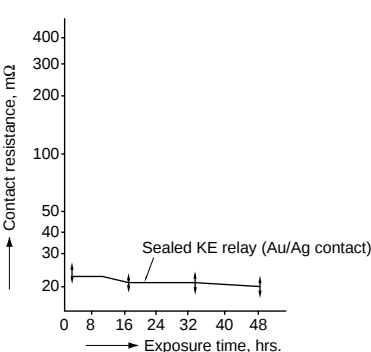
3. H 2 S gas test (1,000 ppm)
