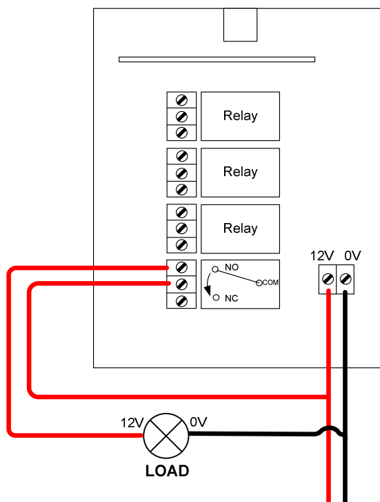
HORNET 12 - 32V Systems 12V Switched Output Example— Only to be used by a competent person
