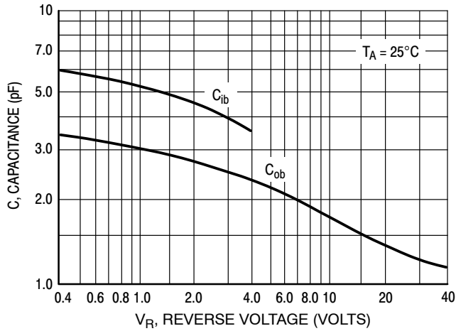
Figure 8. Capacitances
