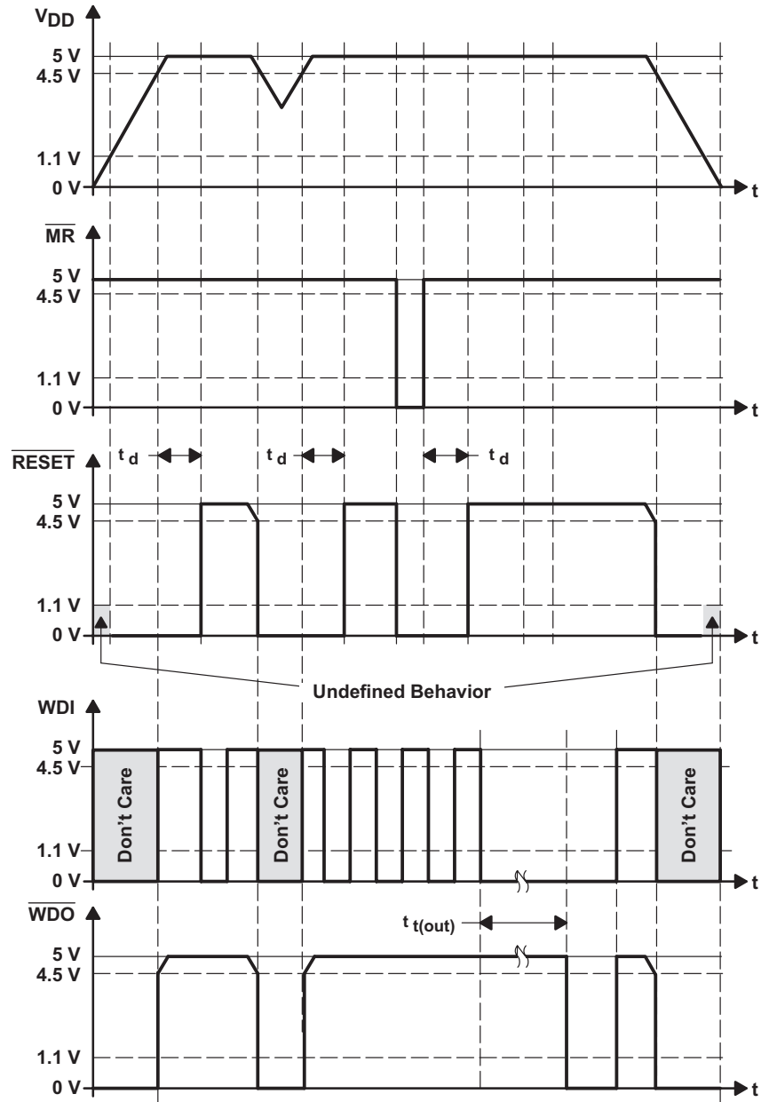
Figure 1. Timing Diagrams
