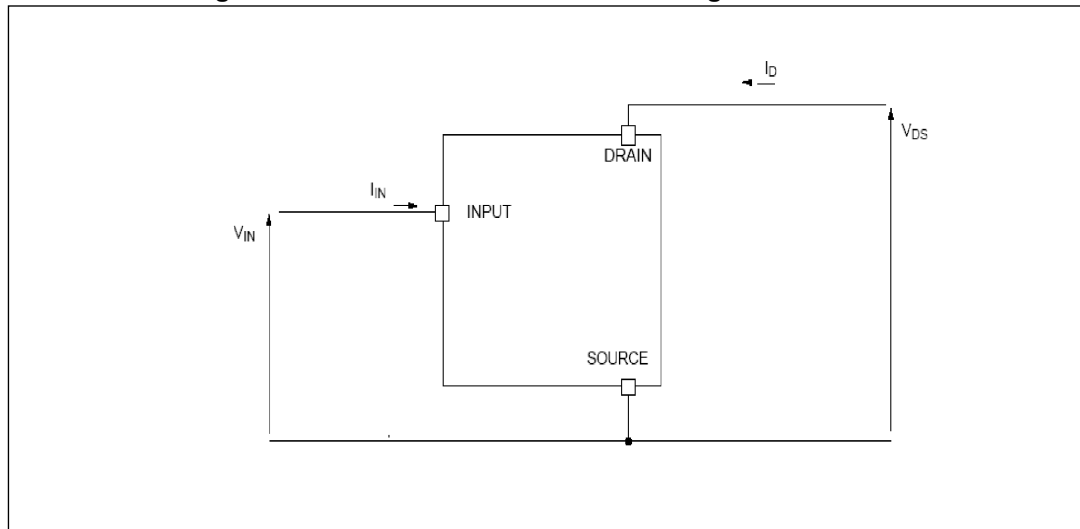
Figure 3. VNL5090N3-E current and voltage conventions
