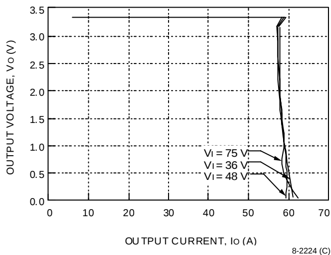
Figure 3. Typical FW250F1 Output Characteristics at Room Temperature
