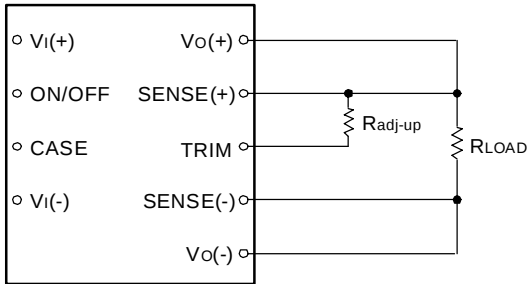
Figure 21. Circuit Configuration to Increase Output Voltage
