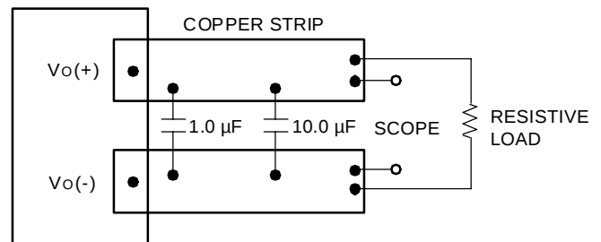
Figure 15. Output Voltage and Efficiency Measurement Test Setup
