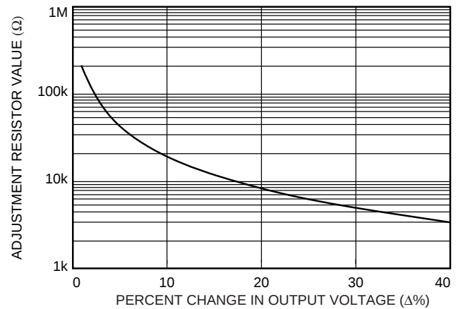
Figure 20. Resistor Selection for Decreased Output Voltage
