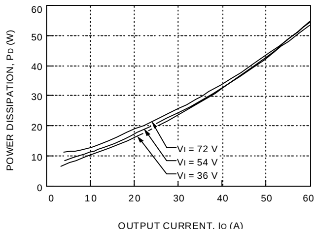
Figure 29. FW250F1 and FW300F1 Power Dissipation vs. Output Current
