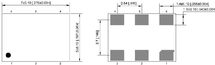
External Dimensions
