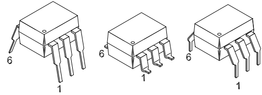
PDIP6 CASE 646BX
