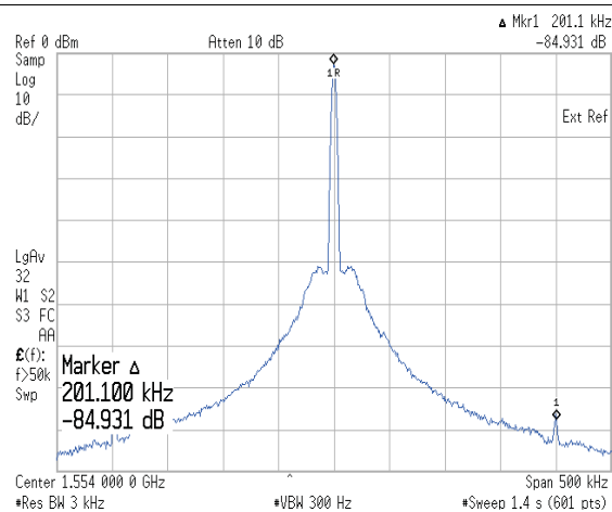
Figure 17. Direct Output: PFD Frequency Spurs
