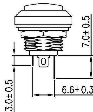
Illuminated Switch
