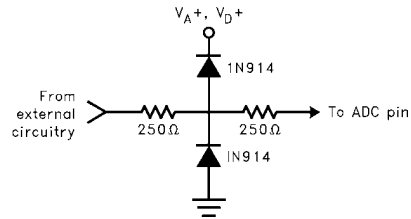
FIGURE 6. Protecting the MUXOUT1, MUXOUT2, A/DIN1 and A/DIN2 Analog Pins
