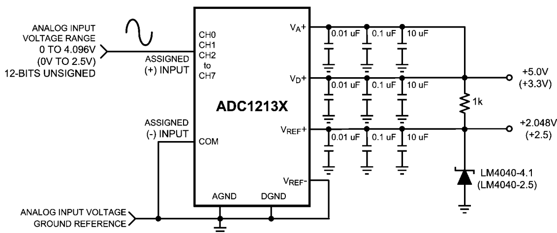
FIGURE 11. Single-Ended Biasing
