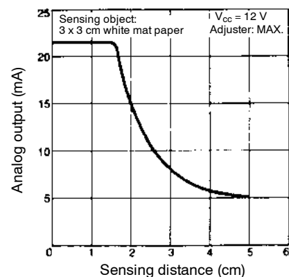
E32-DC200D/D4 with E3XA-CC4A analog amplifier
