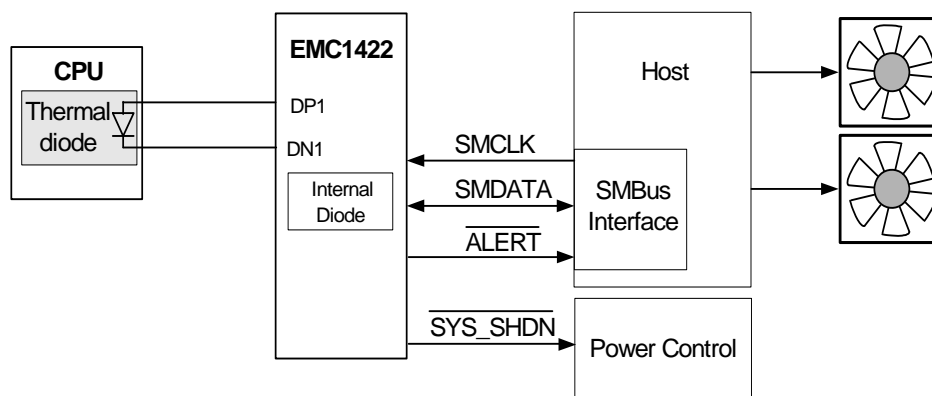
Figure 5.1 System Diagram for EMC1422
