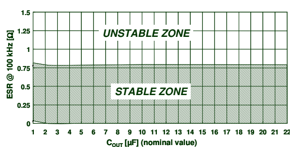
Figure 34. ESR required for stability with ceramic capacitors ( V_{OIT} = 2.5\text{ V} )
