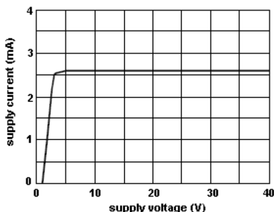
Figure 4. standby supply current vs supply voltage
