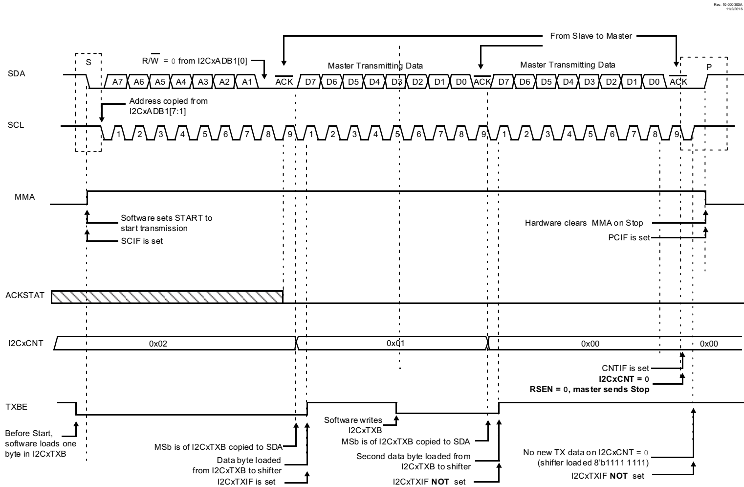
FIGURE 35-19: I 2 C MASTER, 7-BIT ADDRESS, TRANSMISSION WITH STOP
