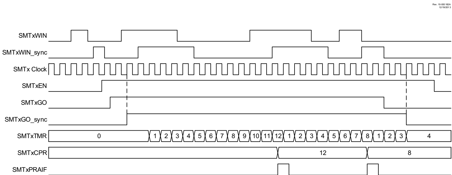
FIGURE 27-10: WINDOWED MEASURE MODE REPEAT ACQUISITION TIMING DIAGRAM
