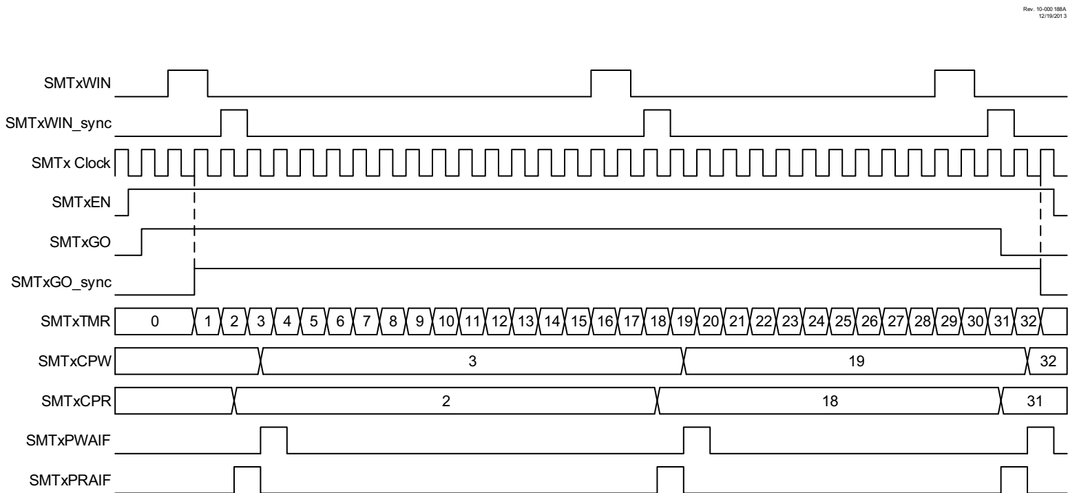
FIGURE 27-16: CAPTURE MODE REPEAT ACQUISITION TIMING DIAGRAM
