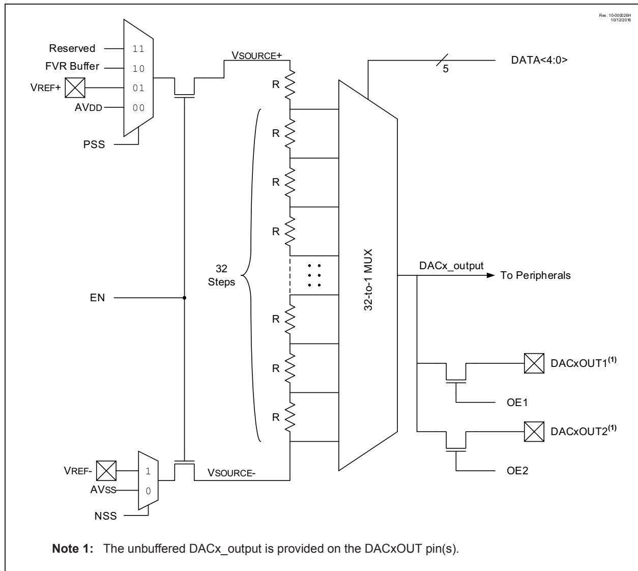
FIGURE 39-1: DIGITAL-TO-ANALOG CONVERTER BLOCK DIAGRAM
