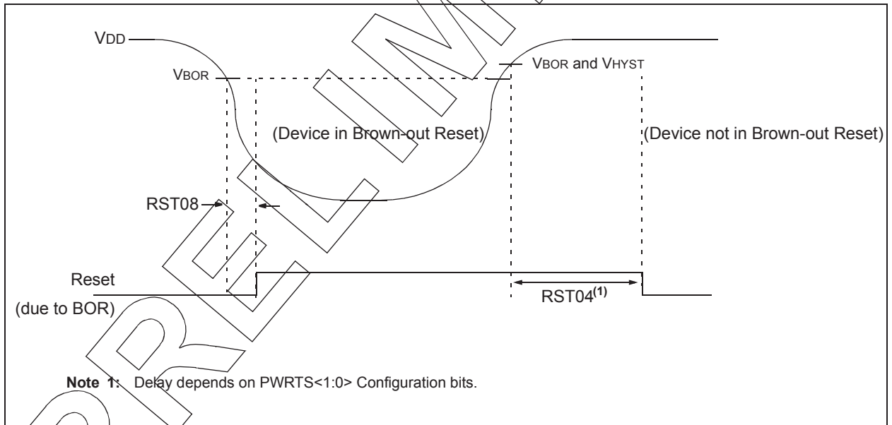
FIGURE 46-9: BROWN-OUT RESET TIMING AND CHARACTERISTICS
