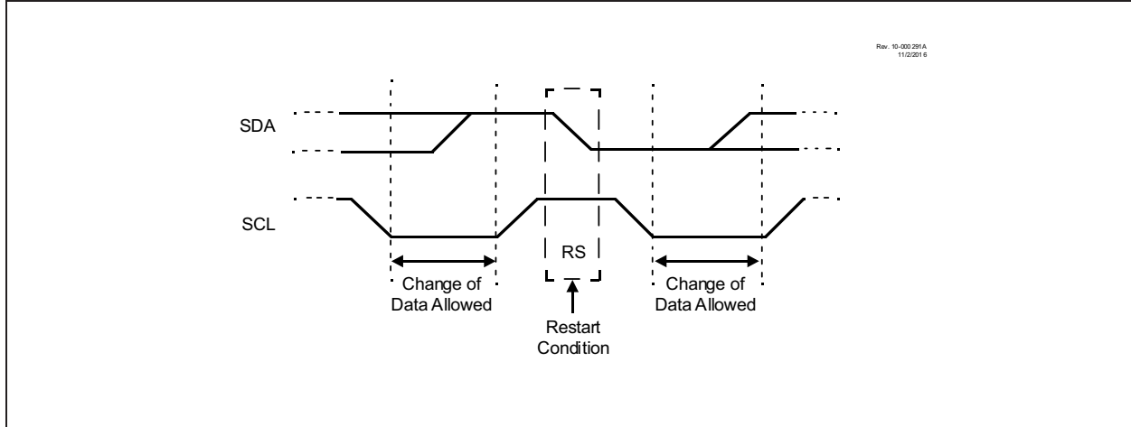
FIGURE 35-4: RESTART CONDITION
