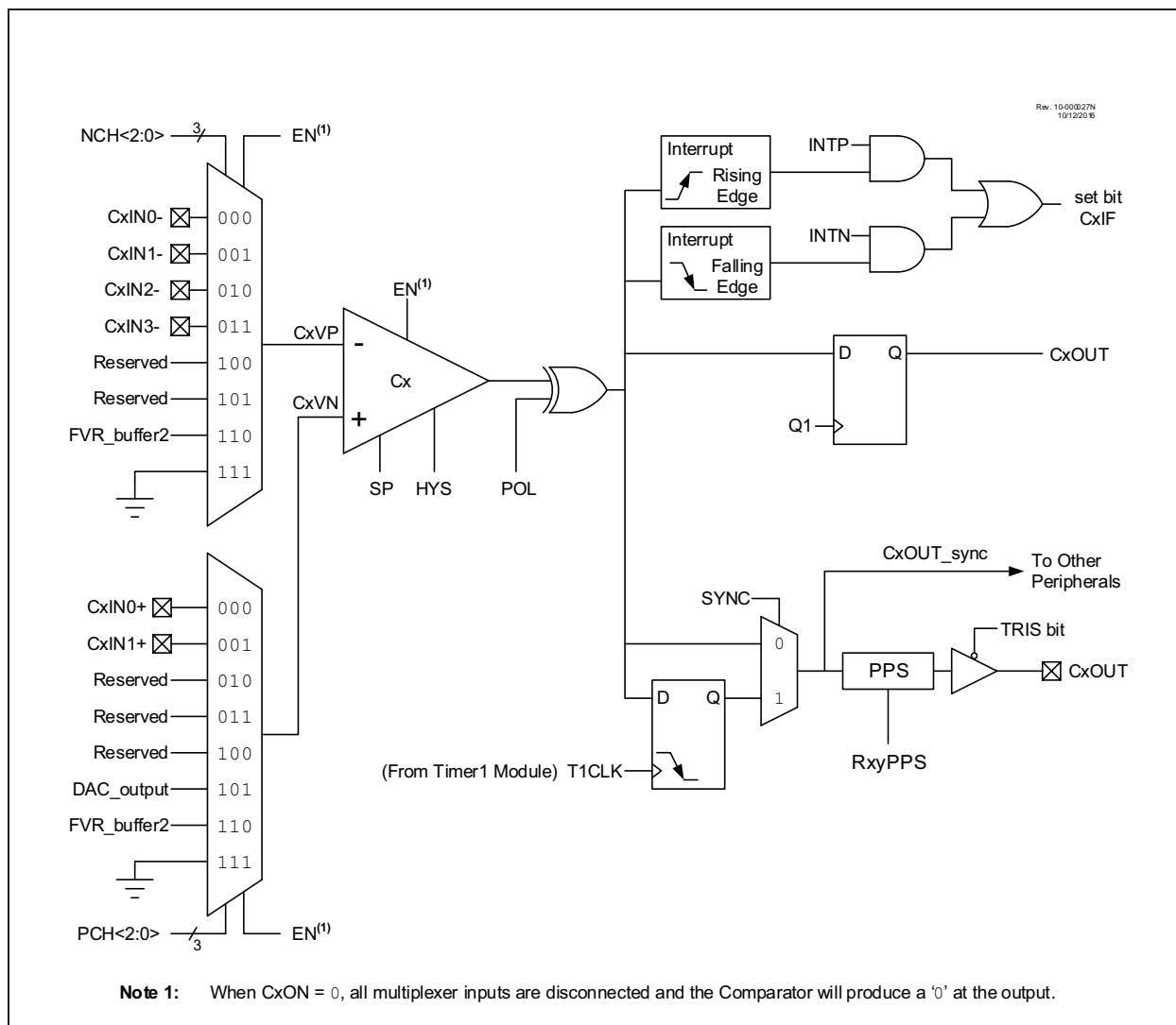
FIGURE 40-2: COMPARATOR MODULE SIMPLIFIED BLOCK DIAGRAM
