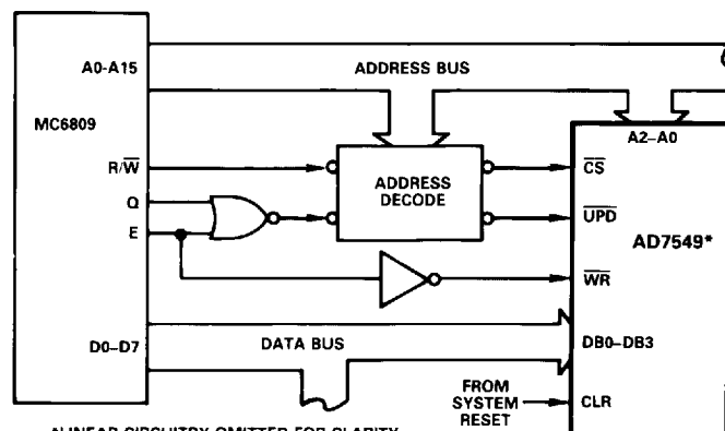
Figure 8. AD7549–MC6809 Interface
