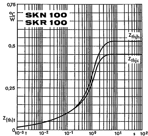
Fig. 5 a Transient thermal impedance vs. time
