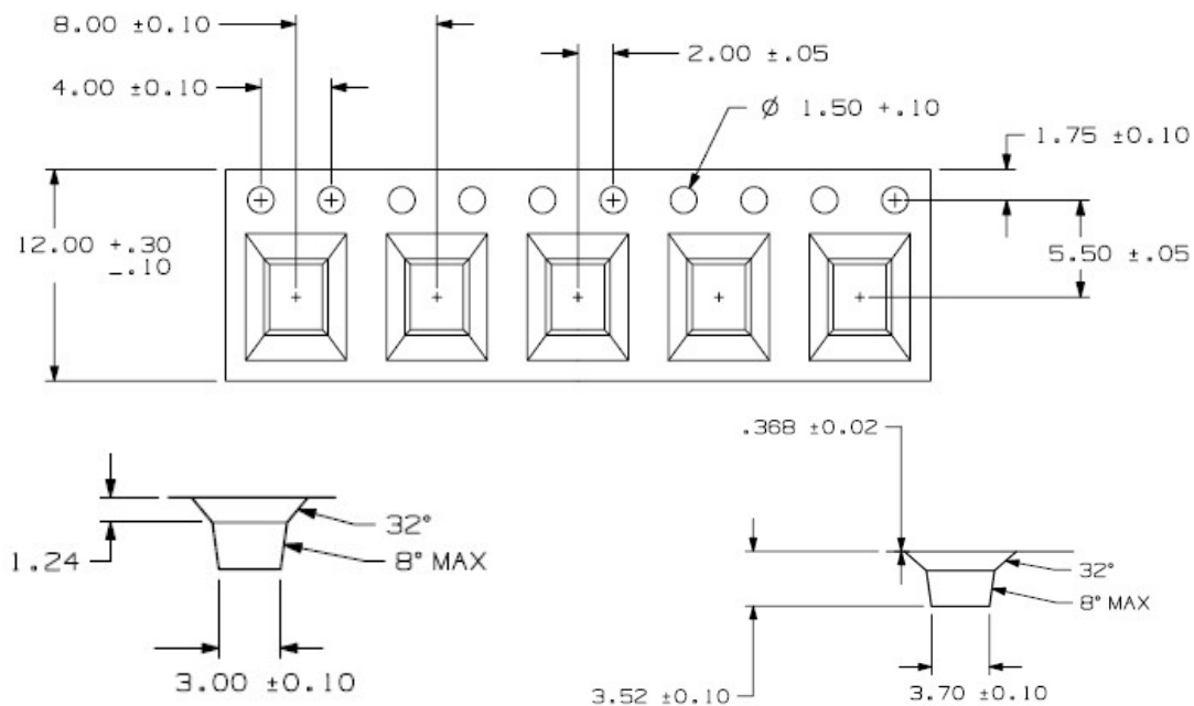
Figure 11. Tape Dimensions
