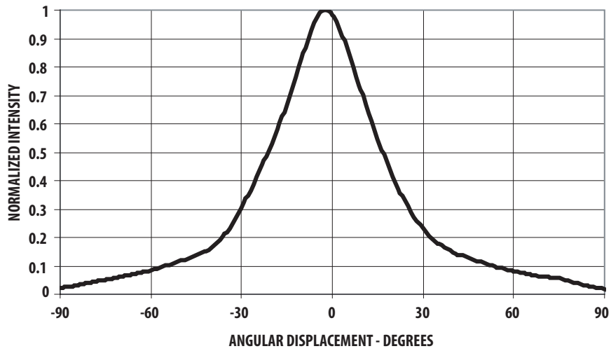
Figure 5. Radiation Pattern
