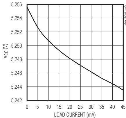
VCC vs. LOAD CURRENT
