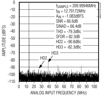
FFT PLOT (8192-POINT DATA RECORD)
