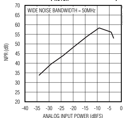
NOISE-POWER RATIO vs. ANALOG INPUT POWER ( f_{NOTCH} = 28.8MHz \pm 1MHz )
