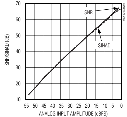
SNR/SINAD vs. ANALOG INPUT AMPLITUDE ( f_{SAMPLE} = 209.99946MHz , f_{IN} = 65.0865033MHz )
