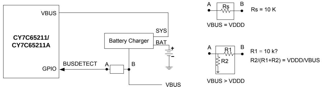
Figure 10. 9 V Tolerant
