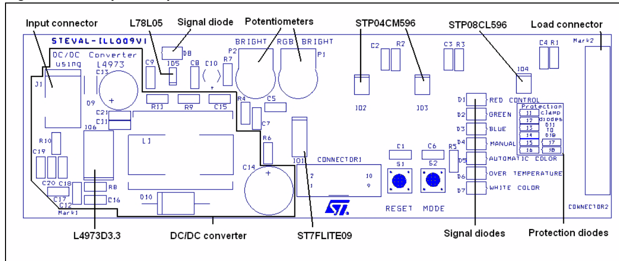
Figure 11. Components position on the STEVAL-ILL009V1
