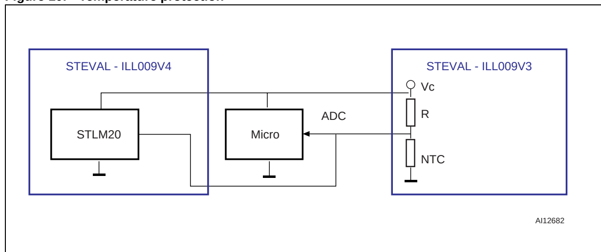
Figure 10. Temperature protection
