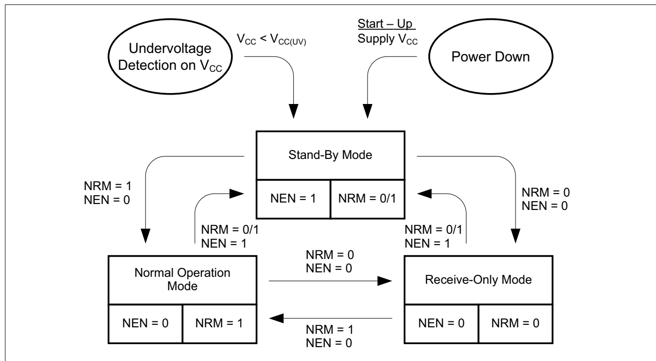
Figure 4 Operation Modes
