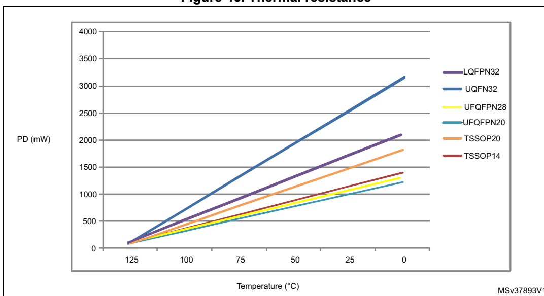
Figure 46. Thermal resistance
