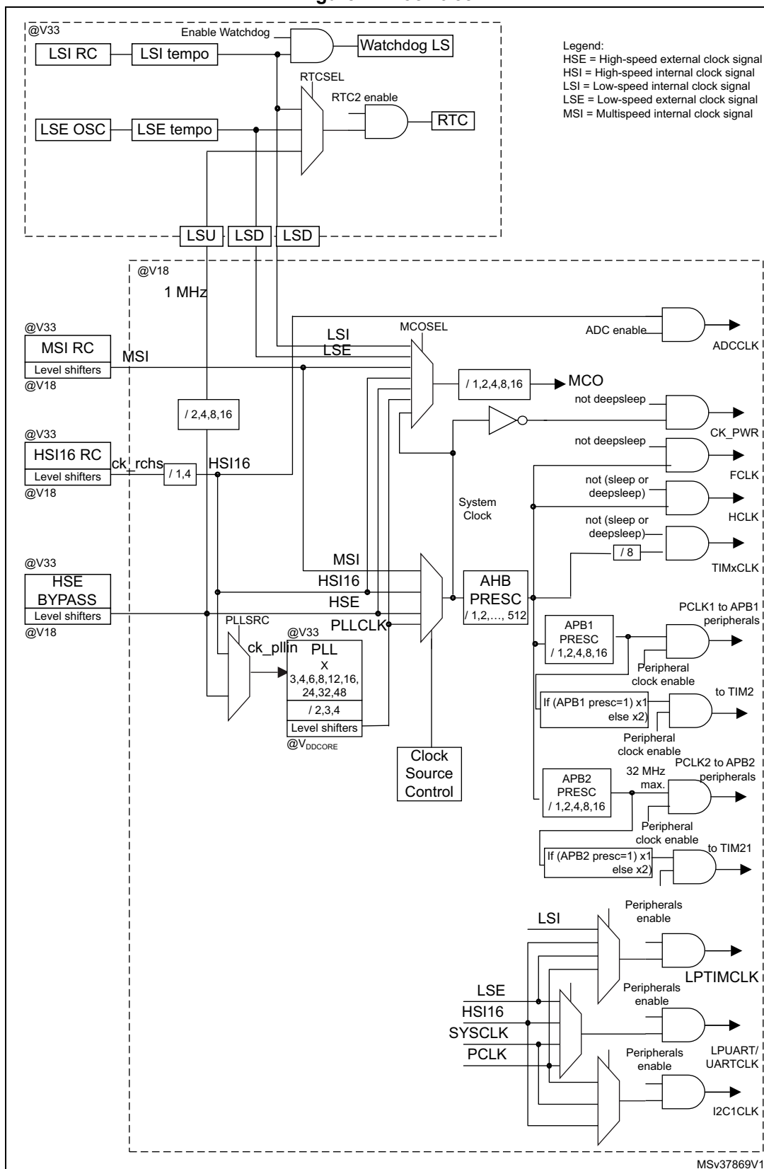
Figure 2. Clock tree
