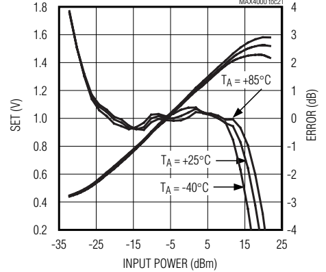
MAX4002 SET AND LOG CONFORMANCE vs. INPUT POWER AT 0.9GHz (UCSP)
