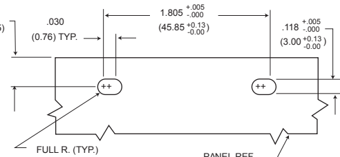
Figure 3 Edgeboard Mounting
