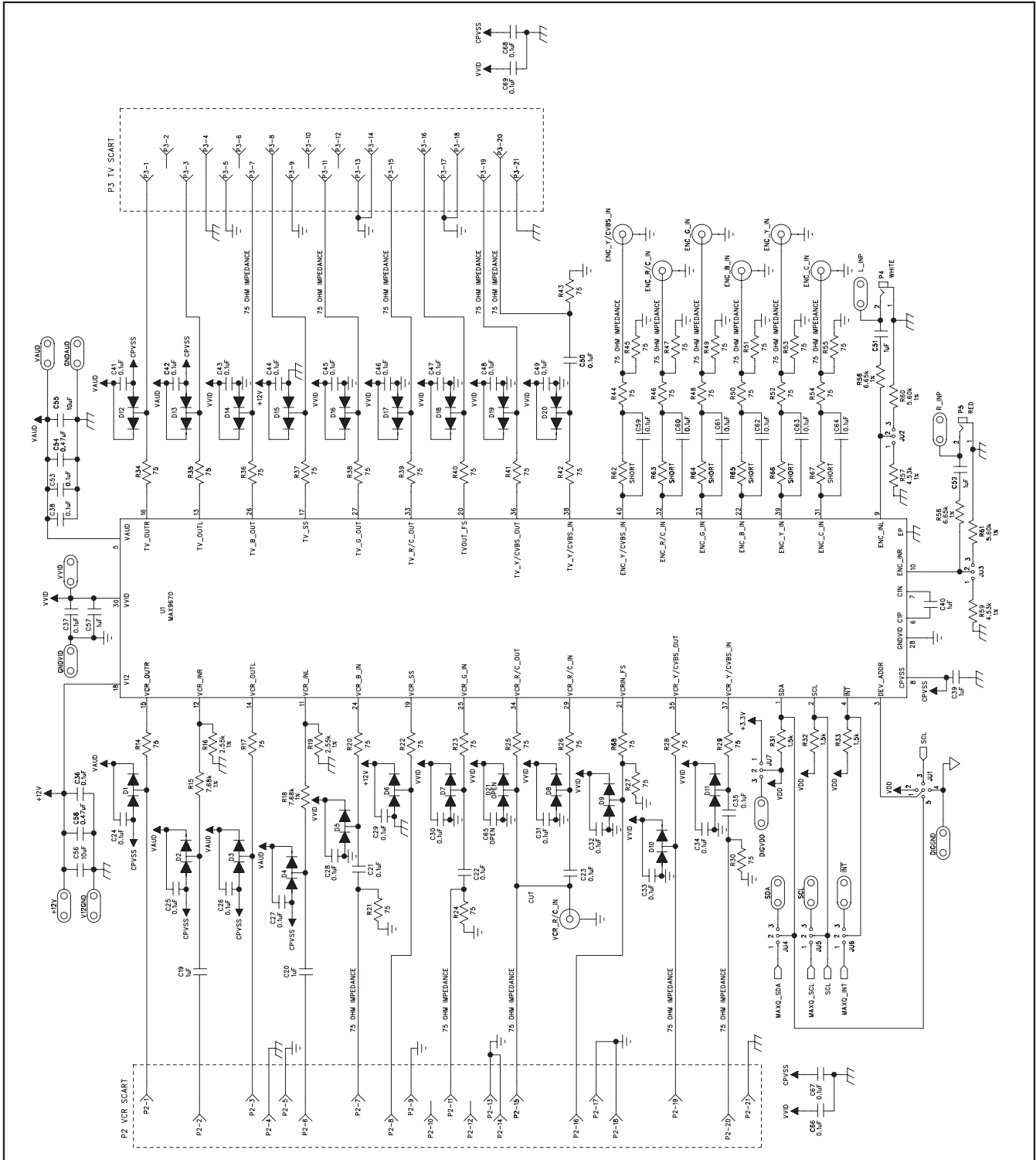
Figure 5a. MAX9670 EV Kit Schematic (Sheet 1 of 2)
