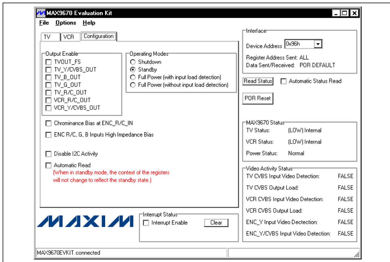
Figure 3. MAX9670 EV Kit Software Main Window (Configuration Control Tab)
