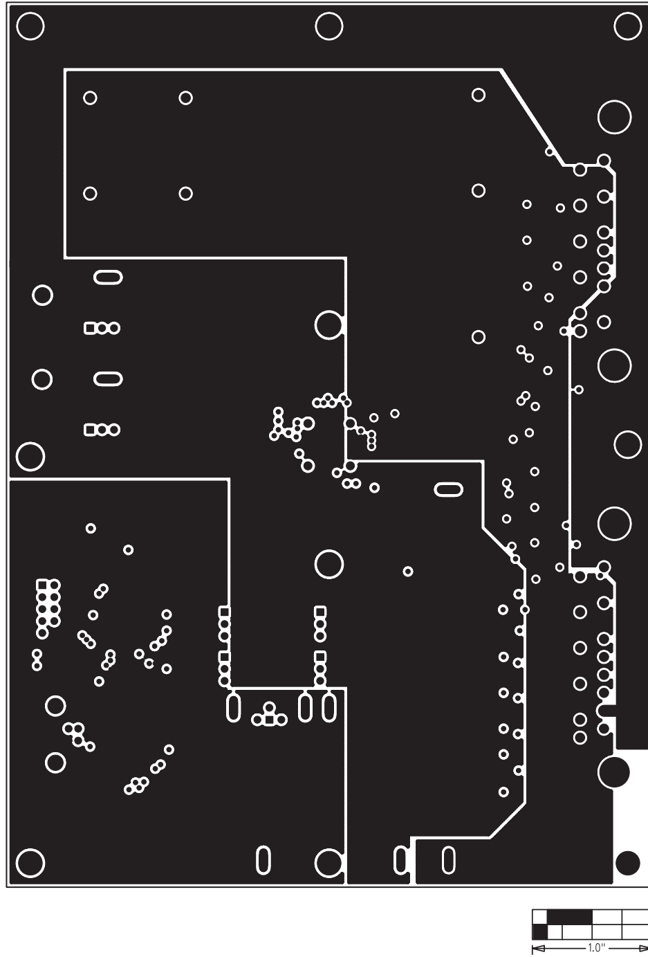
Figure 8. MAX9670 EV Kit PCB Layout—Inner Layer 2
