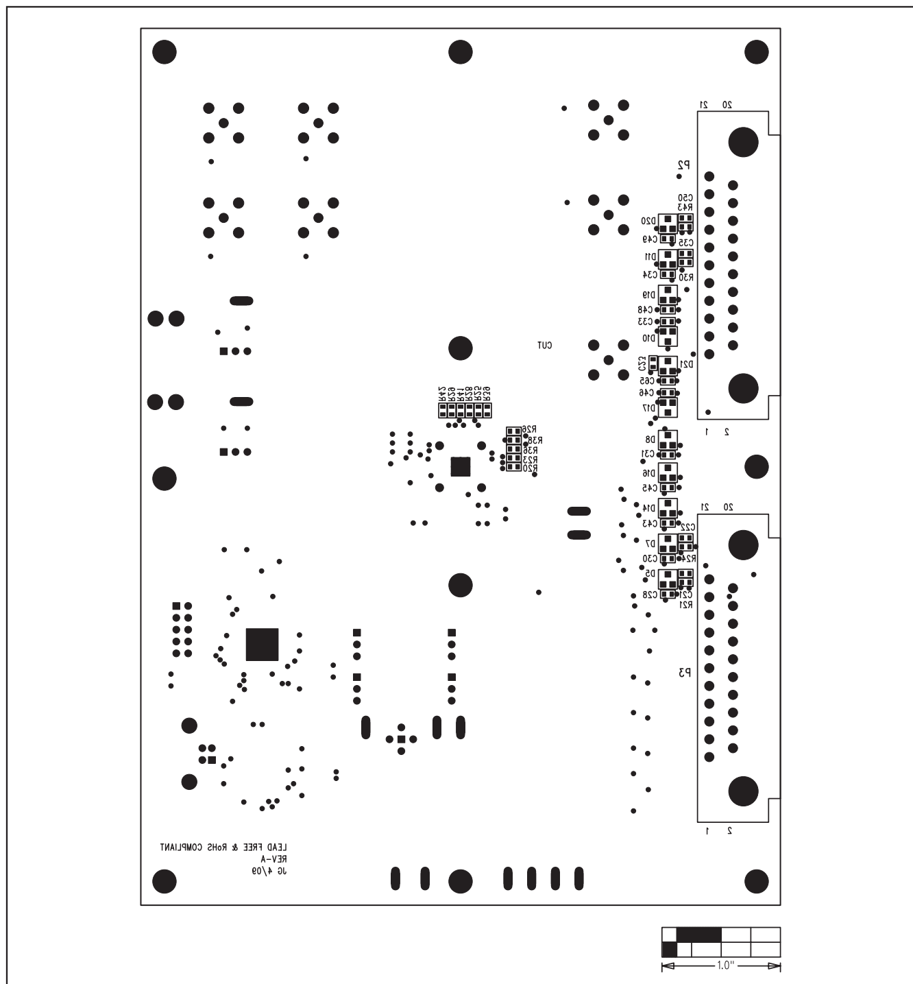
Figure 11. MAX9670 EV Kit Component Placement Guide—Solder Side
