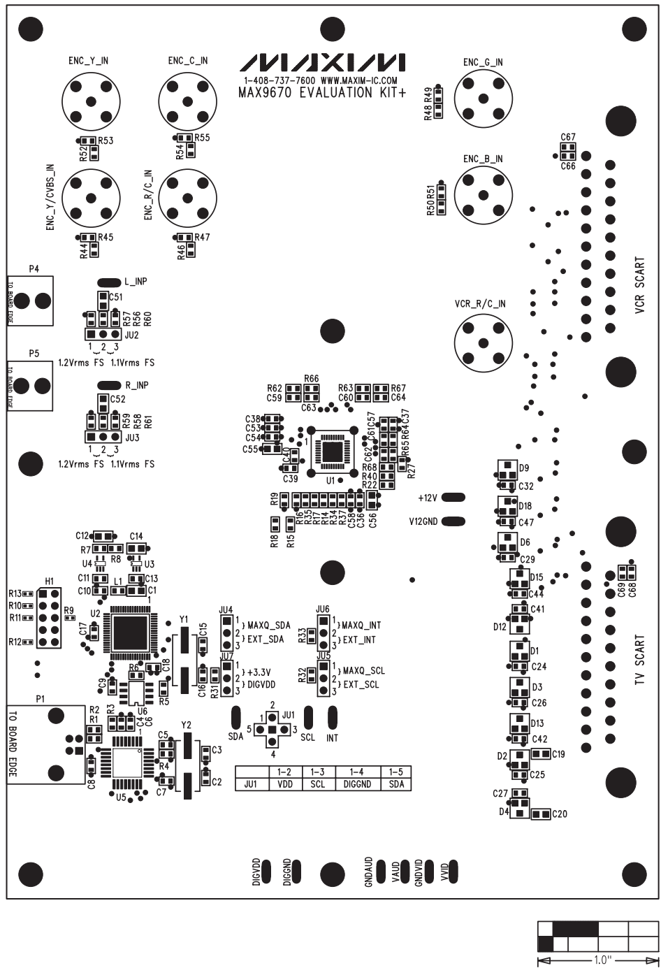
Figure 6. MAX9670 EV Kit Component Placement Guide—Component Side
