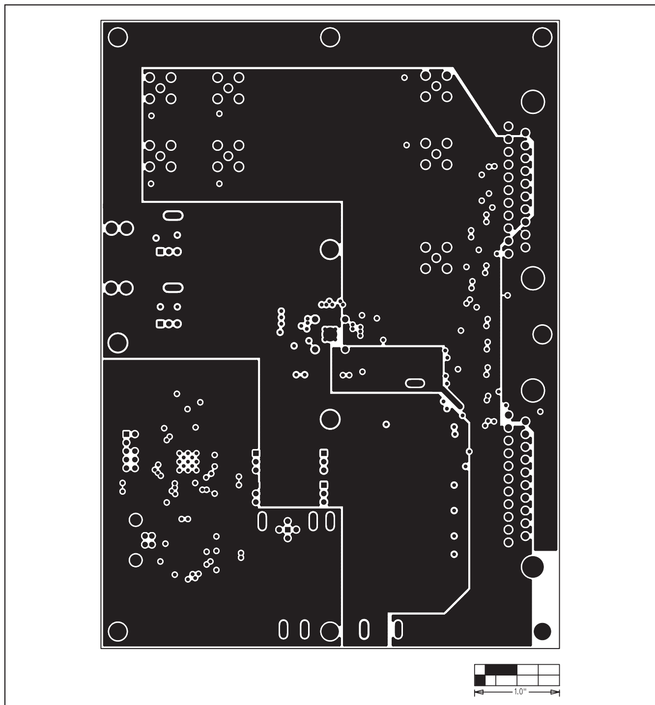
Figure 9. MAX9670 EV Kit PCB Layout—Inner Layer 3
