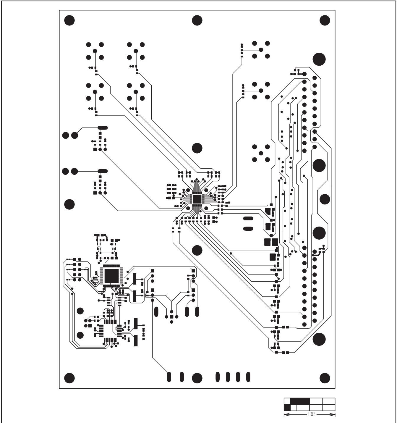
Figure 10. MAX9670 EV Kit PCB Layout—Solder Side
