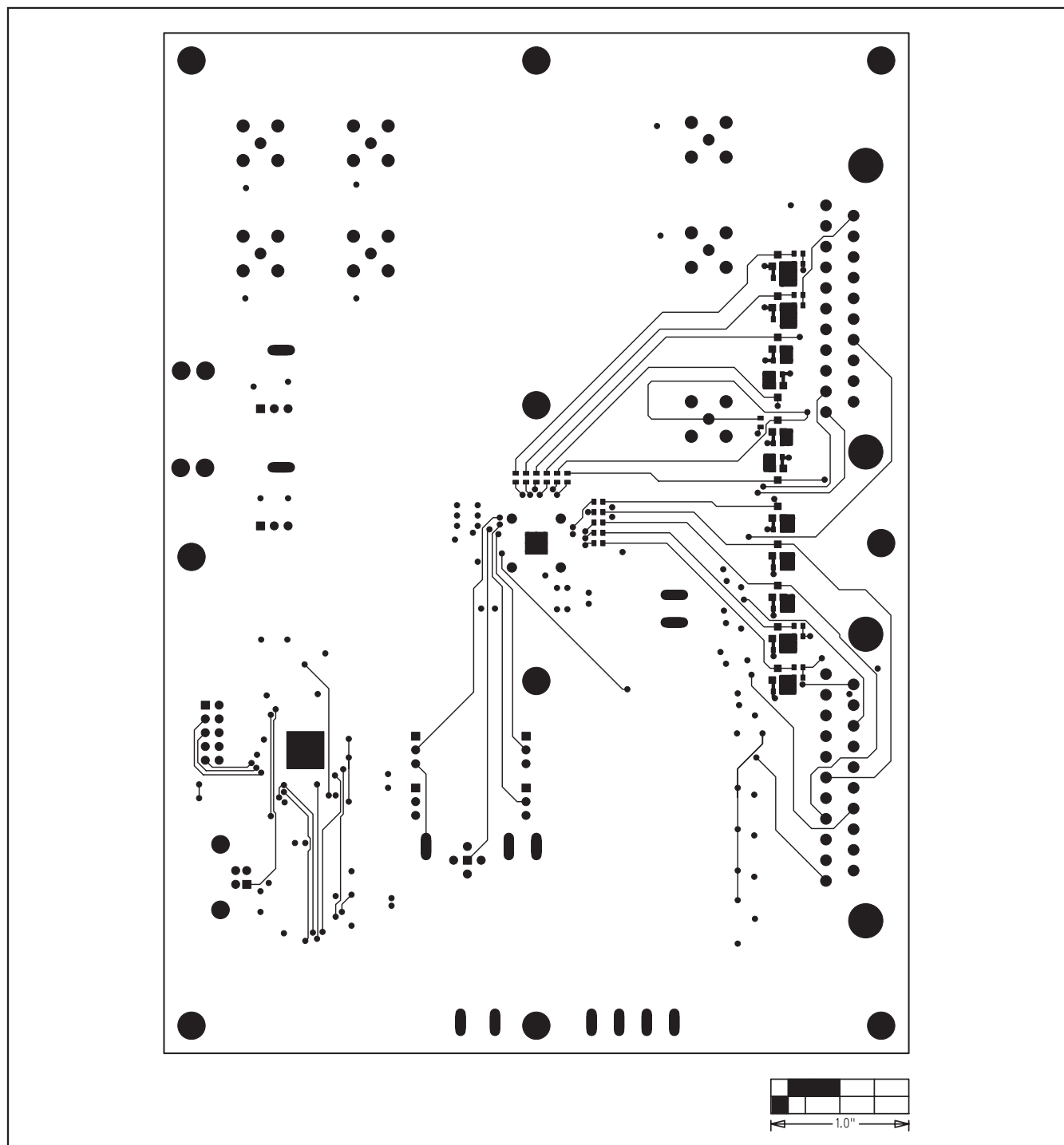
Figure 7. MAX9670 EV Kit Component PCB Layout—Component Side
