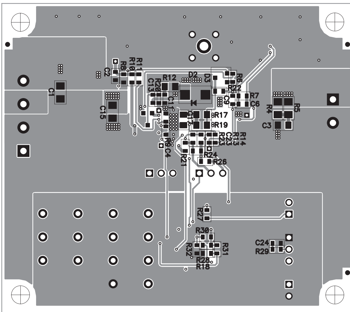
Figure 7. Bottom Assembly
