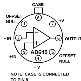
TO-99 (H) Package
