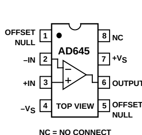
8-Pin Plastic Mini-DIP (N) Package
