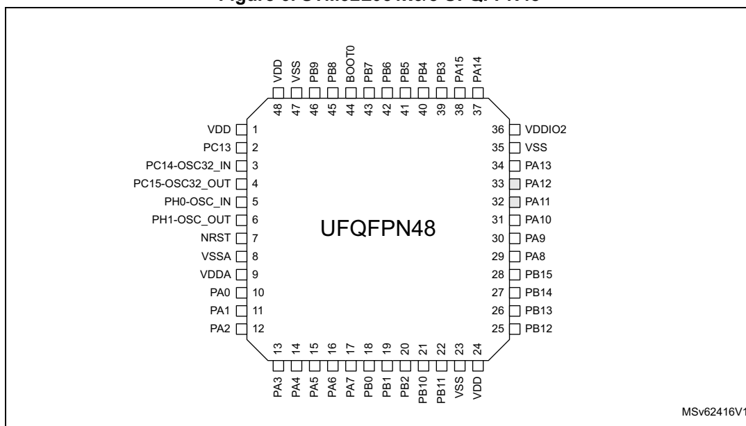
Figure 6. STM32L051x6/8 UFQFPN48
