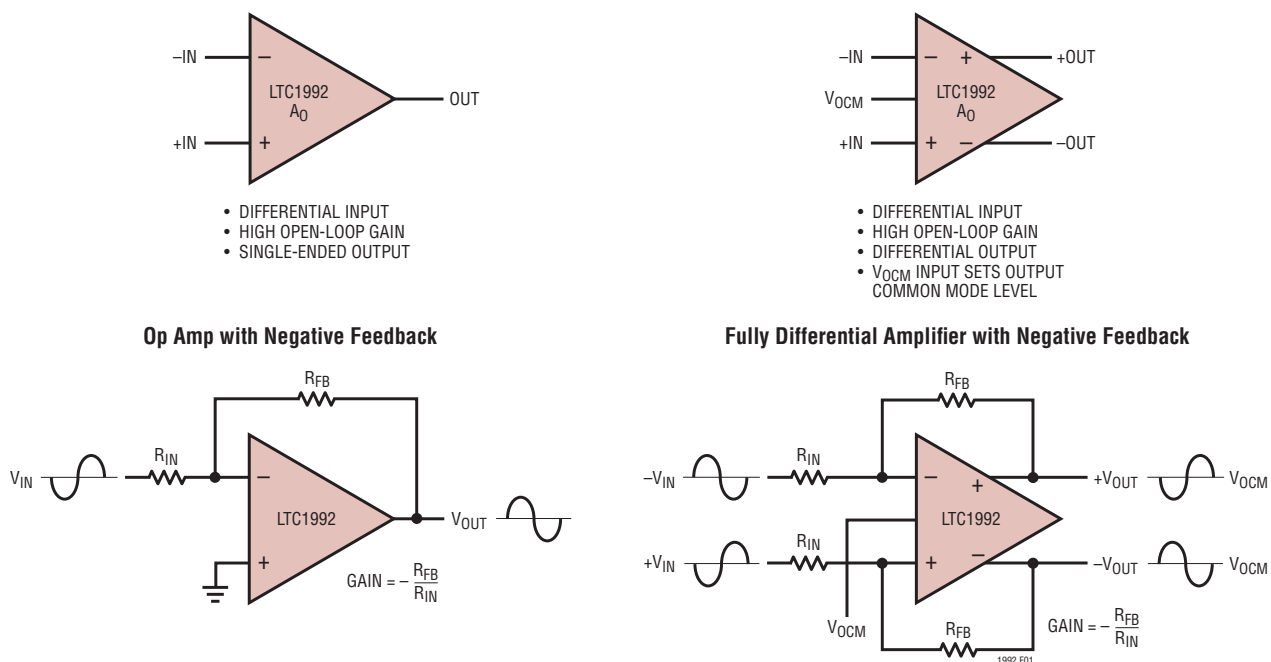
Figure 1. Comparison of an Op Amp and a Fully Differential Amplifier
