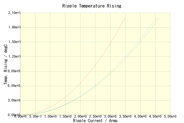
C3225X7R1C106K200AB(100kHz) C3225X7R1C106K200AB(500kHz) C3225X7R1C106K200AB(1MHz)
