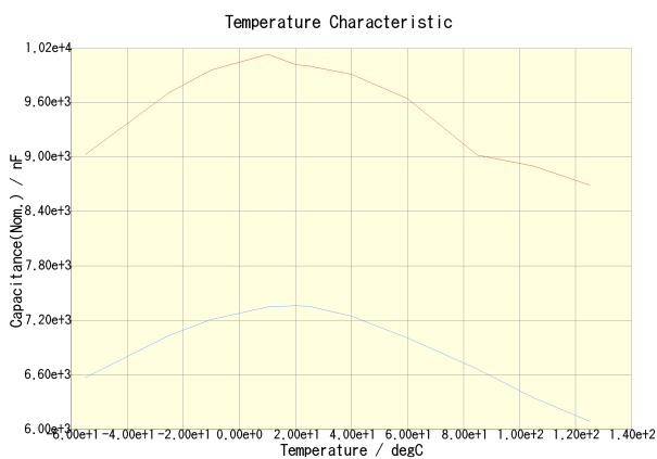
C3225X7R1C106K200AB(DC Bias = 0V) C3225X7R1C106K200AB(DC Bias = 8V)
