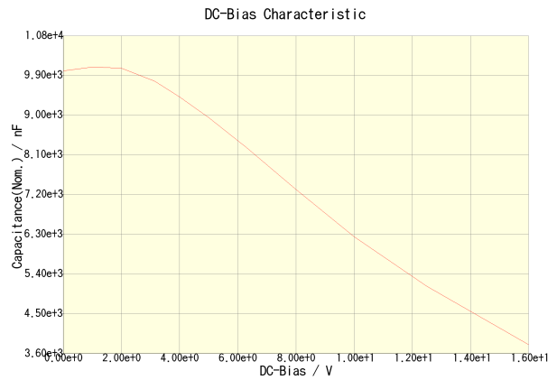
C3225X7R1C106K200AB
