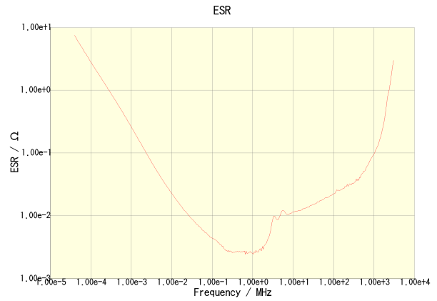
C3225X7R1C106K200AB
