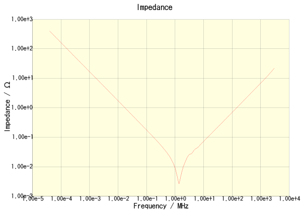
C3225X7R1C106K200AB
