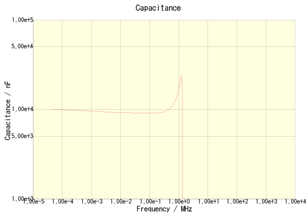
C3225X7R1C106K200AB
