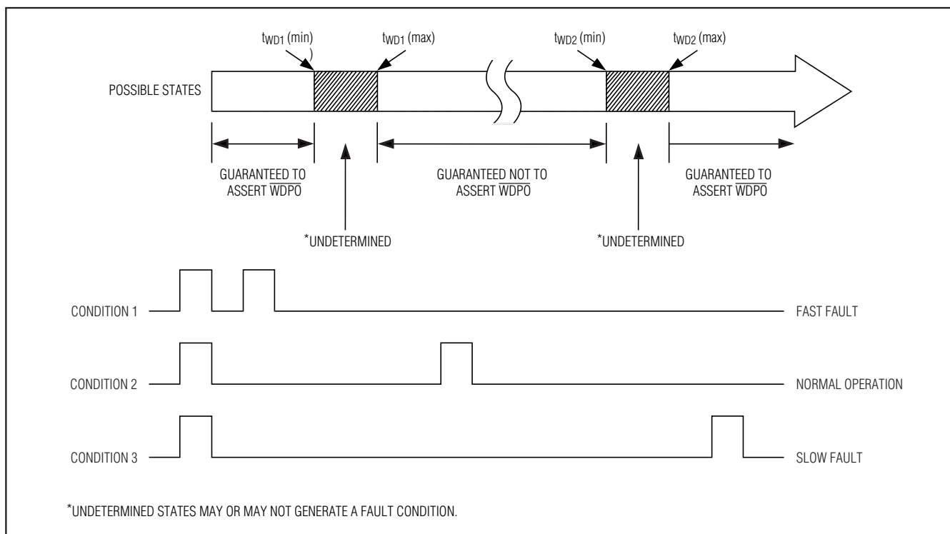
Figure 1. Detailed Watchdog Input Timing Relationship
