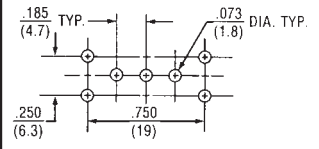
1 Pole P.C. Mounting
