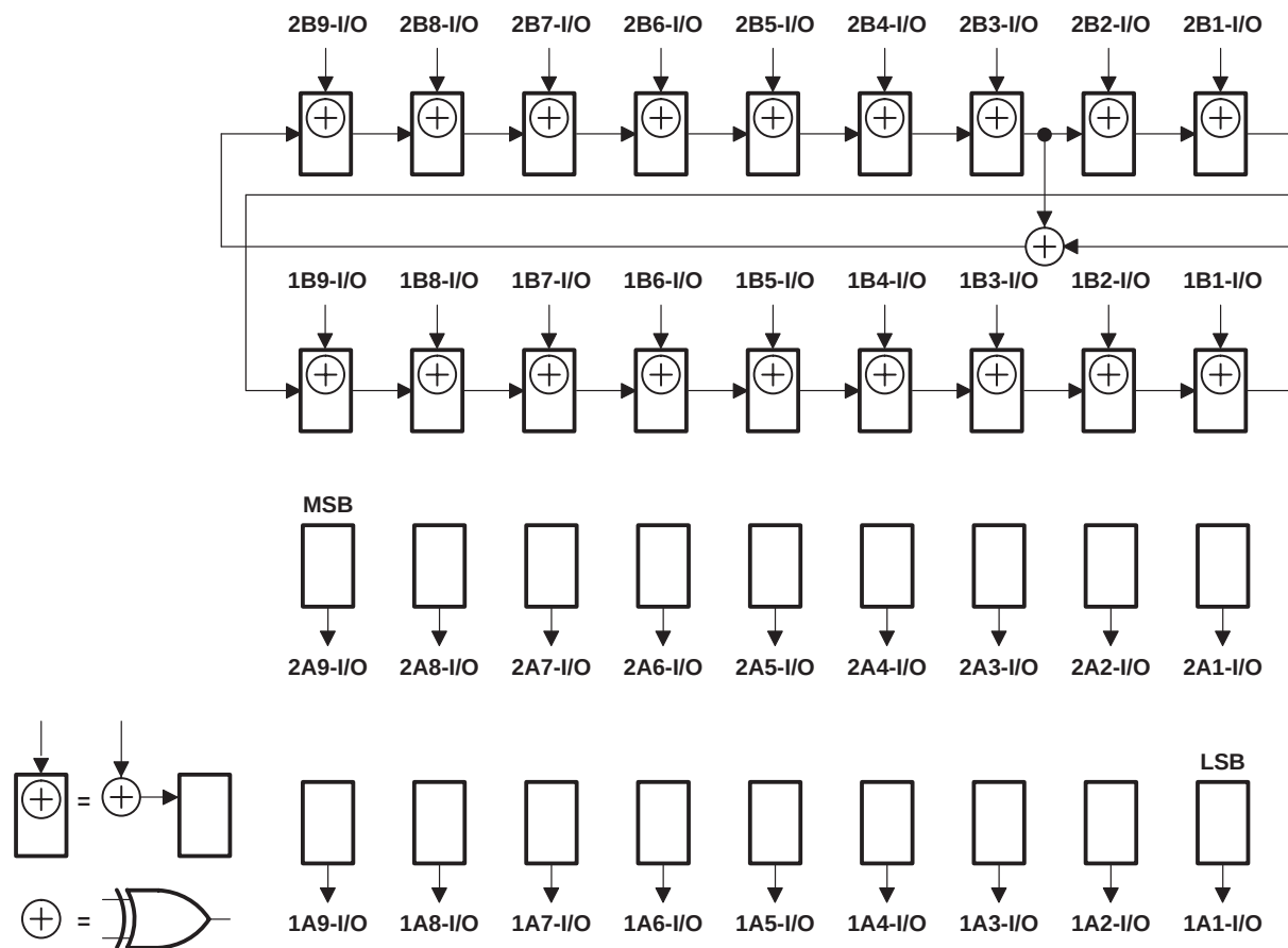
Figure 13. 18-Bit PSA/COUNT Configuration (10EAB = 20EAB = 0, \overline{10EBA} = \overline{20EBA} = 0 )
