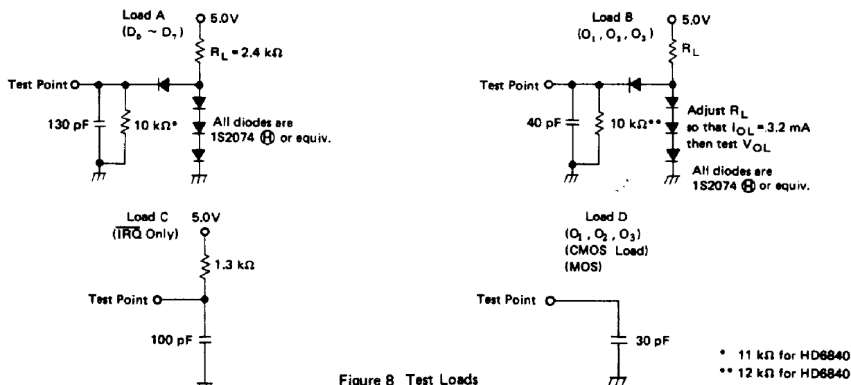
Figure 8 Test Loads
