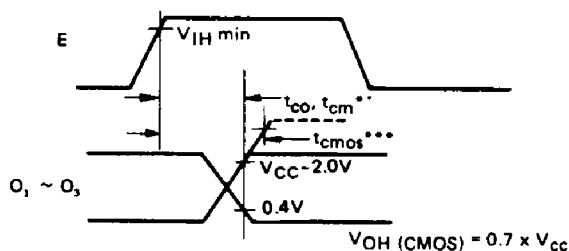
Figure 6 Output Delay
