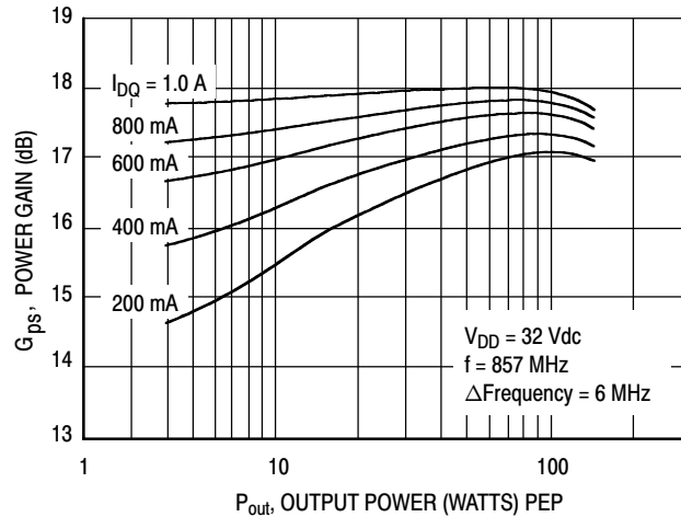
Figure 9. Power Gain versus Peak Output Power in Narrowband Circuit
