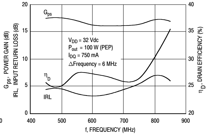
Figure 5. Performance in Broadband Circuit
