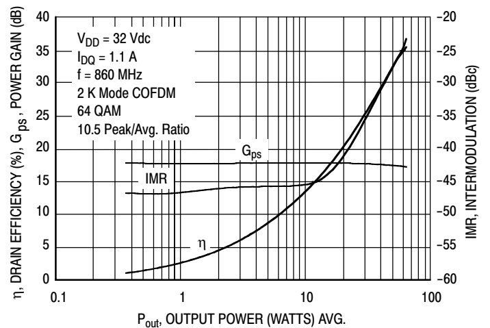
Figure 7. COFDM Intermodulation, Gain and Efficiency versus Output Power in Broadband Circuit
