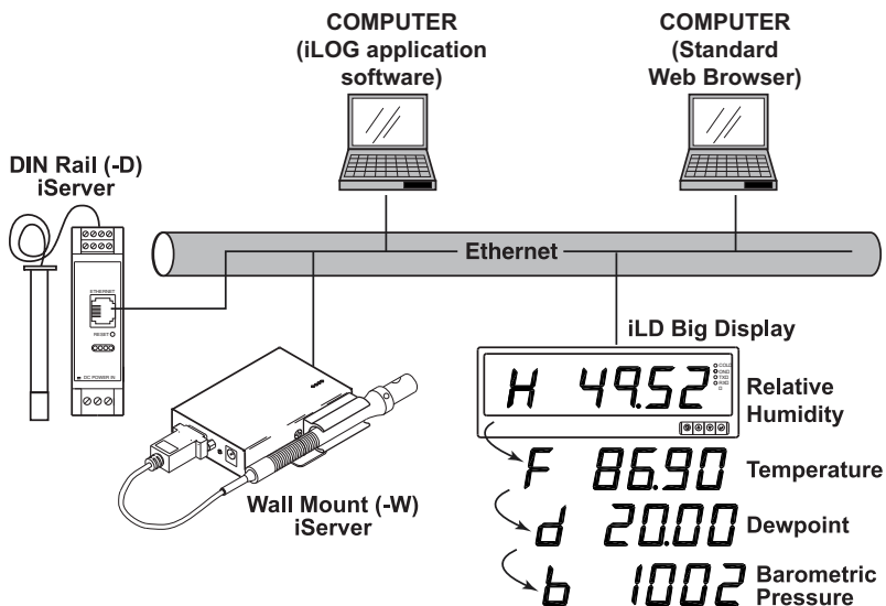
Figure 1.1 iServer with Probe on the Ethernet Network
