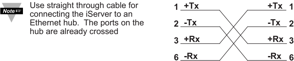
Figure 2.5 10Base-T Crossover Cable Wiring
