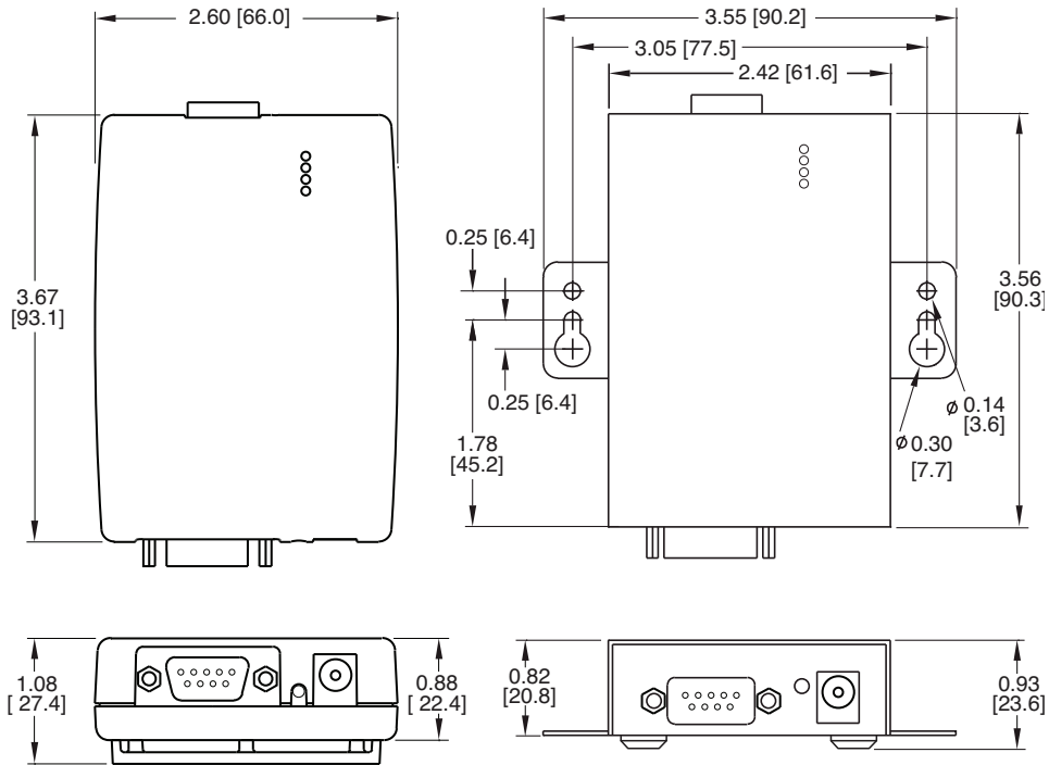
Version A - new case style Version B - older case style Figure 5.1 Wall Mount iServer Dimensions
