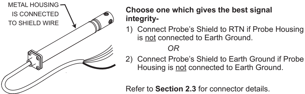
Figure 2.6 Industrial Probe Wiring Hookup
