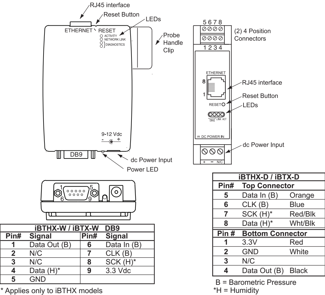
Figure 2.3 Parts of the iServer Unit
