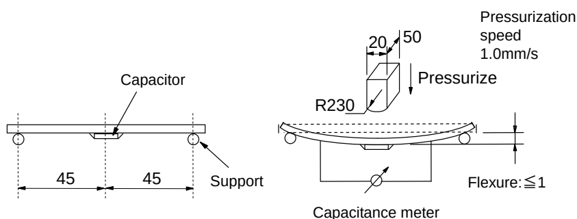
Fig.2 (in mm)
