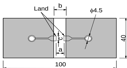
Fig.1 (in mm)
